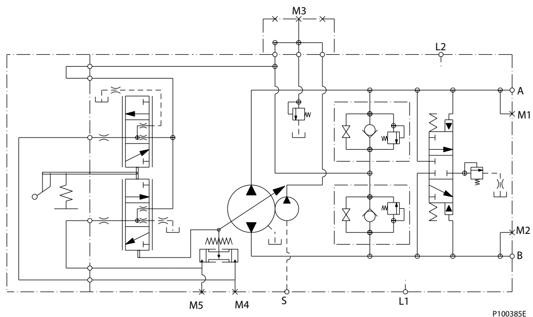
Schematic Diagram
