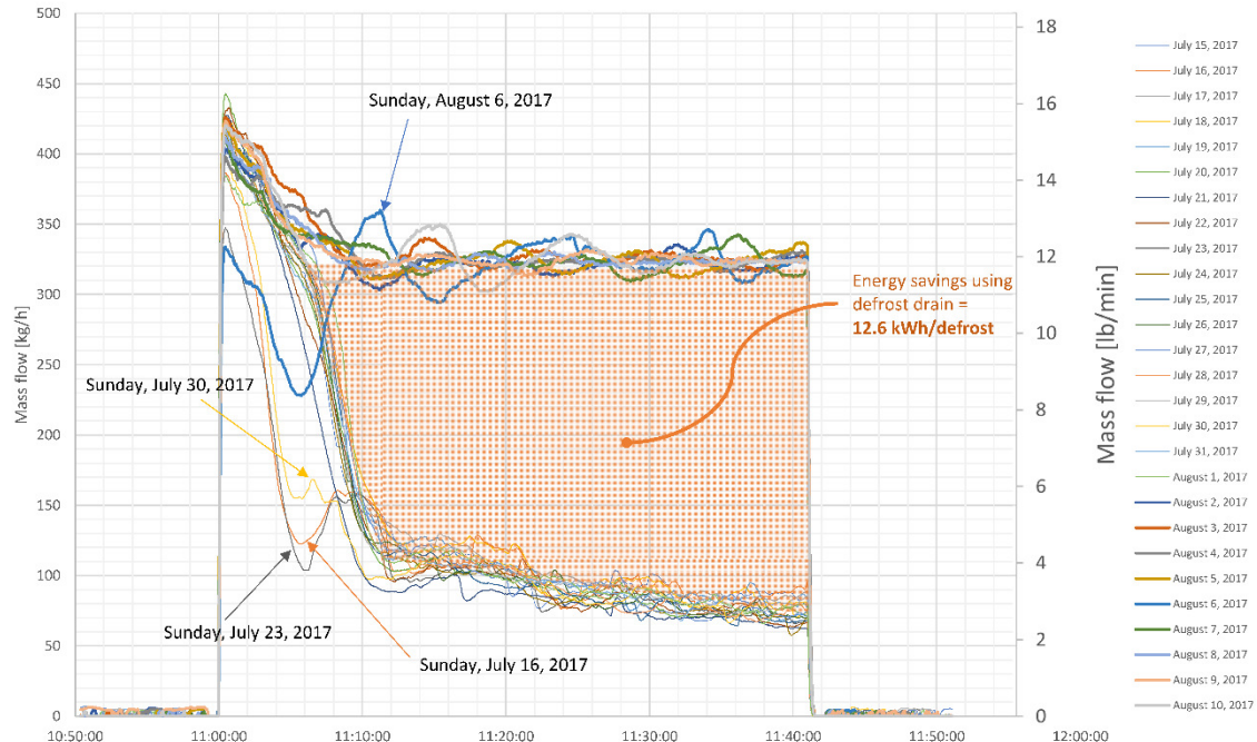
Figure 13: Field test results from a European customer test site: Hot gas mass flow from old Pressure Control system vs. the new Danfoss ICFD Defrost Module based on the Liquid Drain method.
