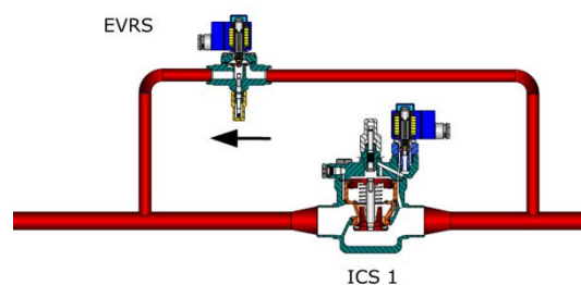
Figure 16: Example of "Soft opening solenoid solution"
