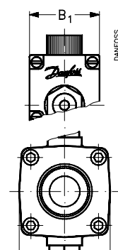
EVRA 32 and 40 Coil with terminal box
