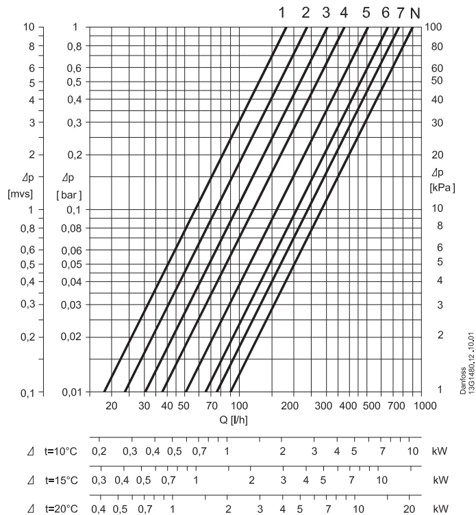
RA-N 013G7382 – Capacities at X_p = 2K
