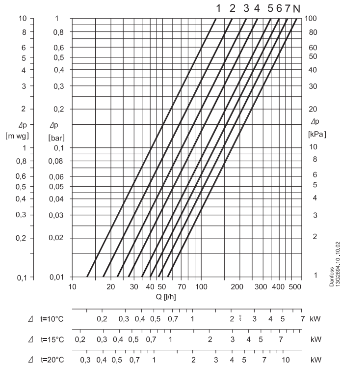
RA-N 013G7382 – Capacities at X_p = 1K
