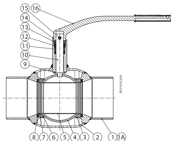
DN 65-80 with handle
