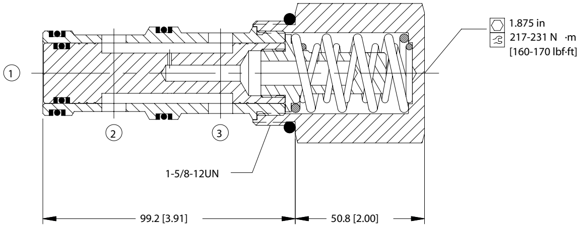
Cross-sectional view
