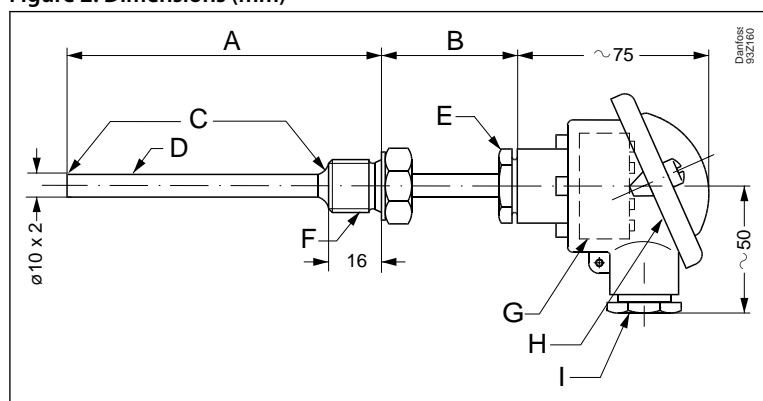
Figure 2: Dimensions (mm)
