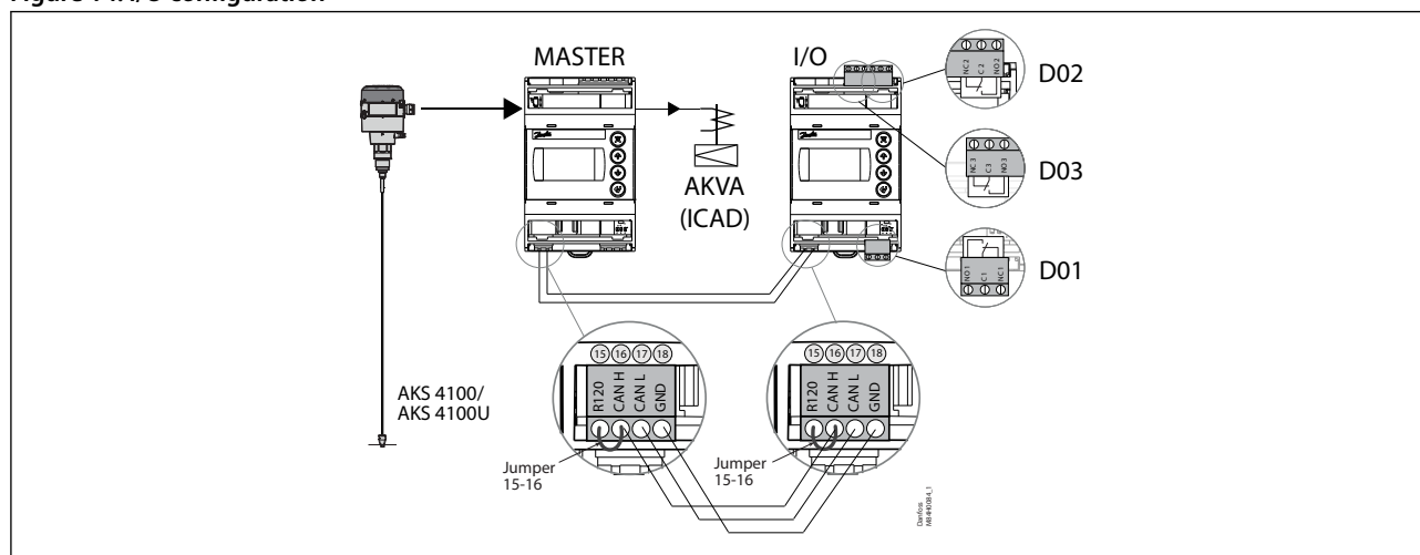
Figure 14: I/O configuration
