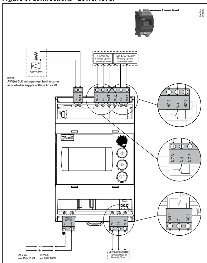
Figure 6: Connections - Lower level
