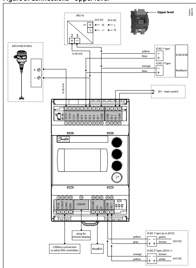
Figure 5: Connections - Upper level
