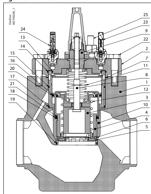
Figure 5: ICLX 100-150
