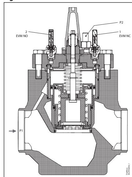
Figure 2: ICLX 100-150
