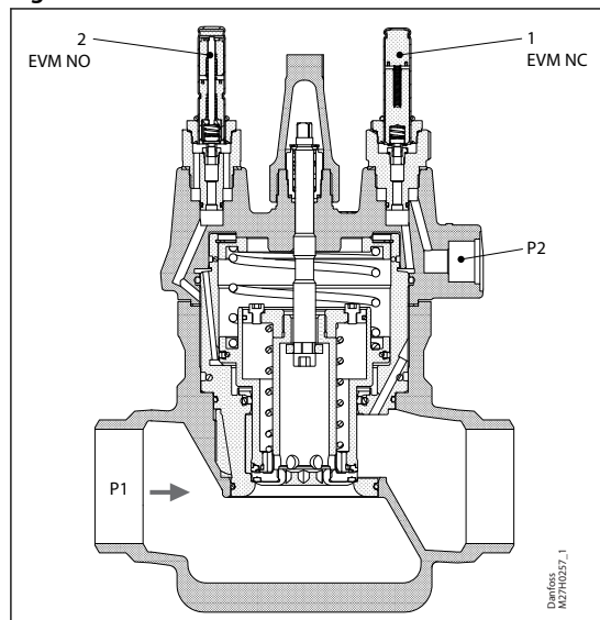
Figure 1: ICLX 32-65
