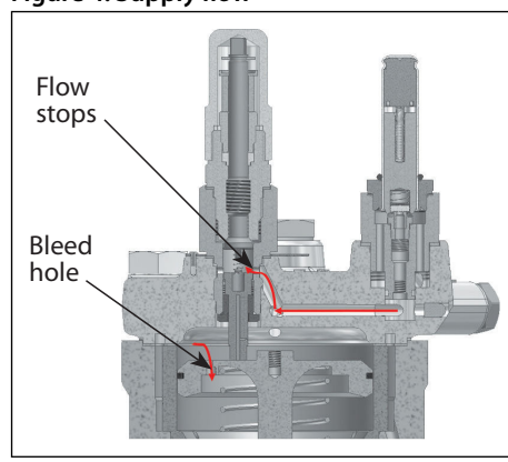
Figure 4: Supply flow
