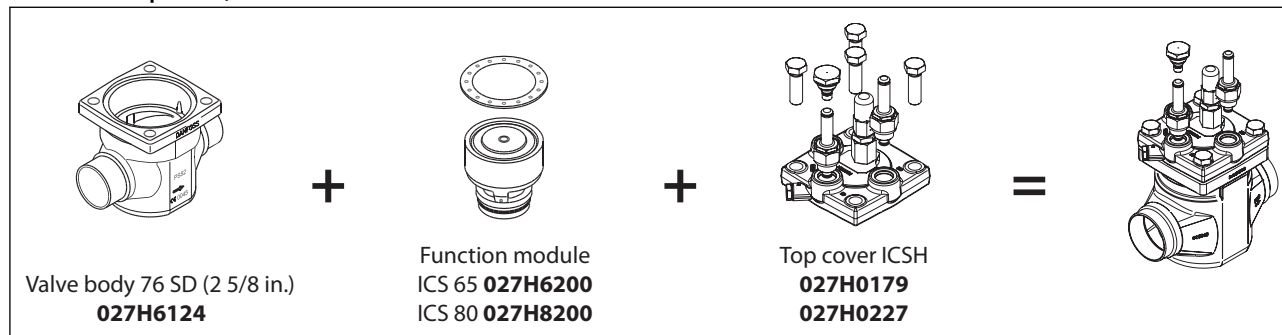
Figure 35: ICV 65 valve body
