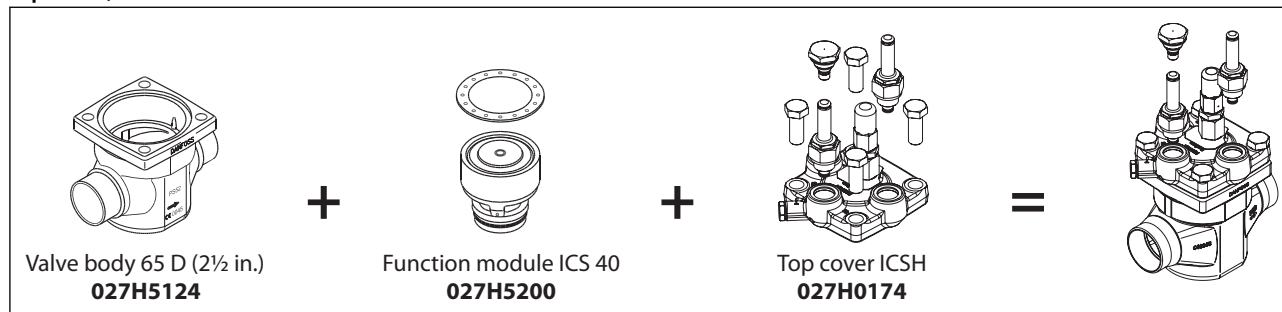
Figure 30: ICV 50 valve body
