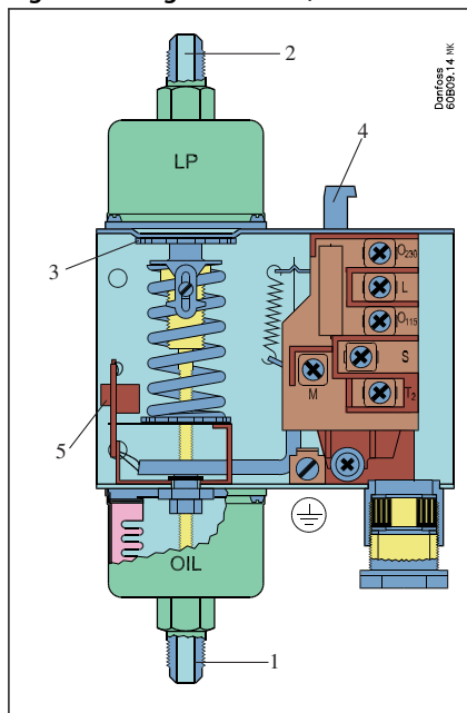
Figure 4: Design for MP 54, MP 55 and MP 55A
