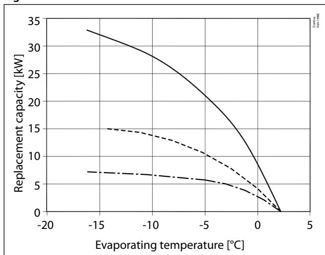
Figure 15: TGHE - R404A/R507
