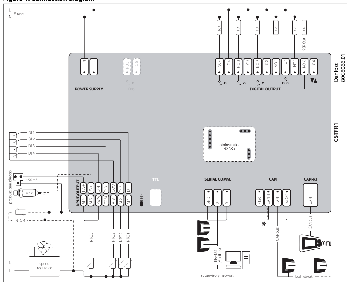
Figure 1: Connection diagram
