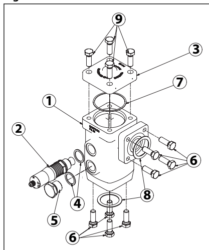
Figure 4: Material AKS 38 Retrofit housing
