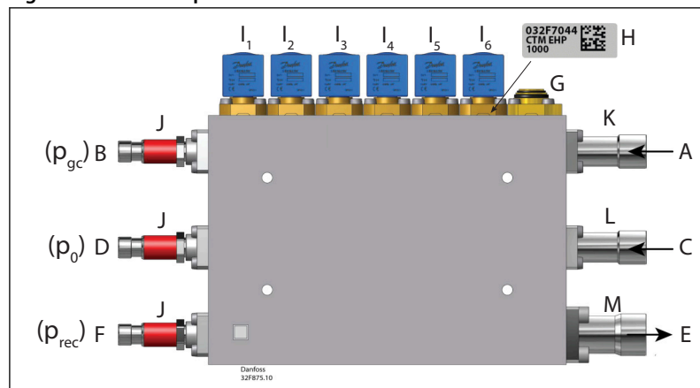
Figure 5: Connector positions
