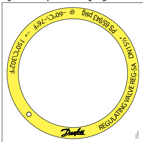
Figure 5: Example of marking ring, REG-SA
