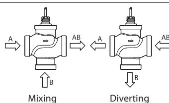
Fig. 1: Mixing or diverting connection
