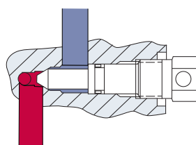
Bypass valve
