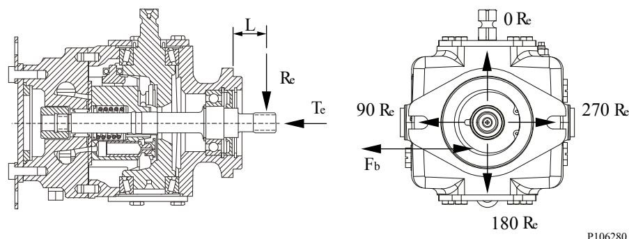
Diagram of external radial shaft loads
