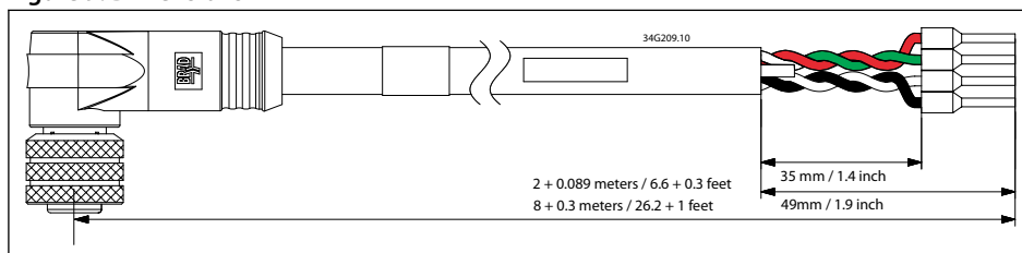
Figure 9: Dimensions
