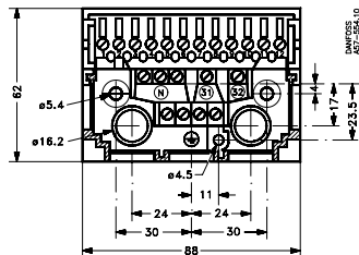
Embase 057H7210
