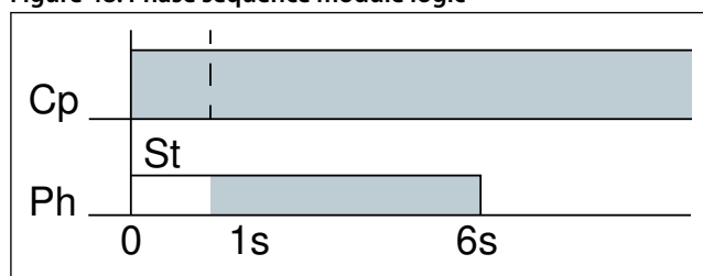
Figure 48: Phase sequence module logic
