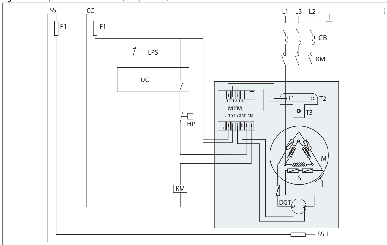
Figure 61: Compressor model DSH485 (except code 3) and model DSH600
