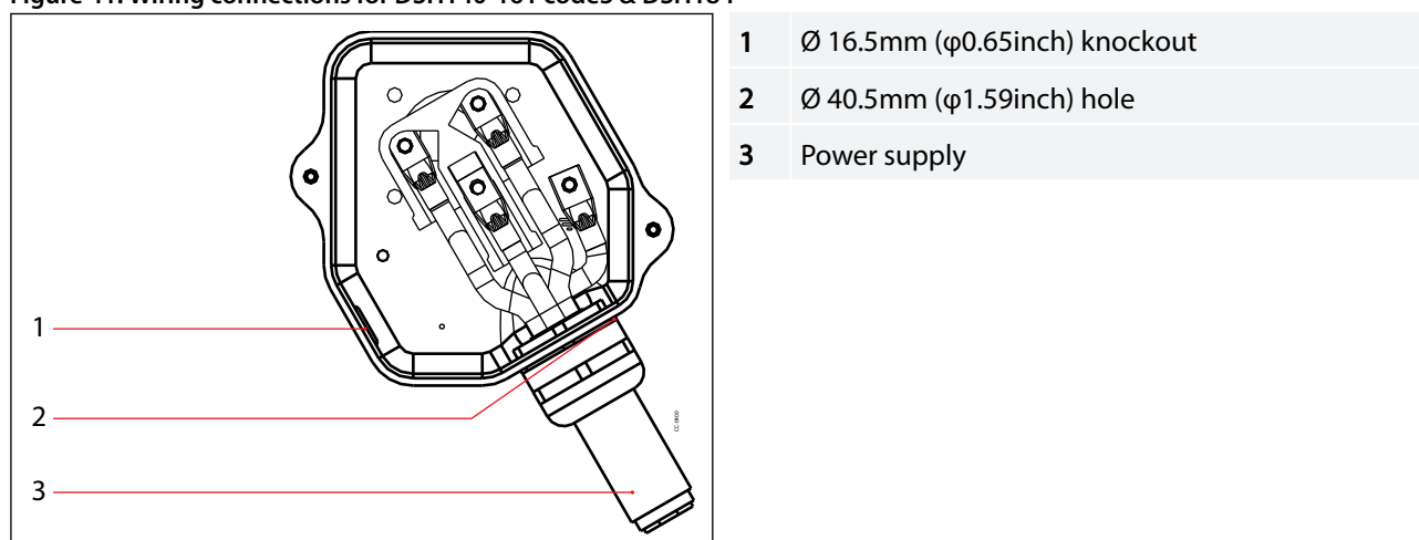
Figure 41: Wiring connections for DSH140-161 code3 & DSH184
