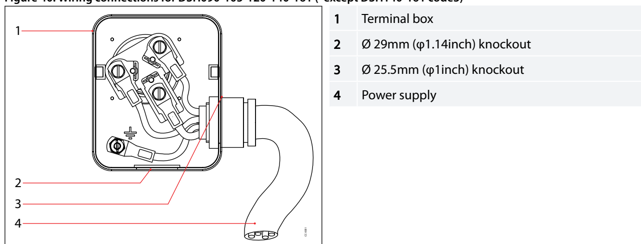
Figure 40: Wiring connections for DSH090-105-120-140-161 (*except DSH140-161 code3)
