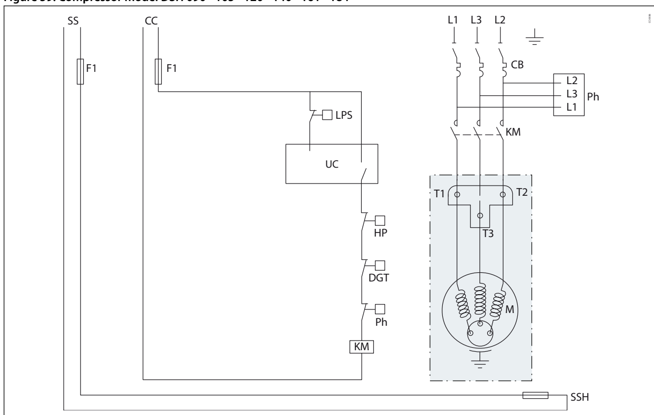
Figure 59: Compressor model DSH 090 - 105 - 120 - 140 - 161 - 184
