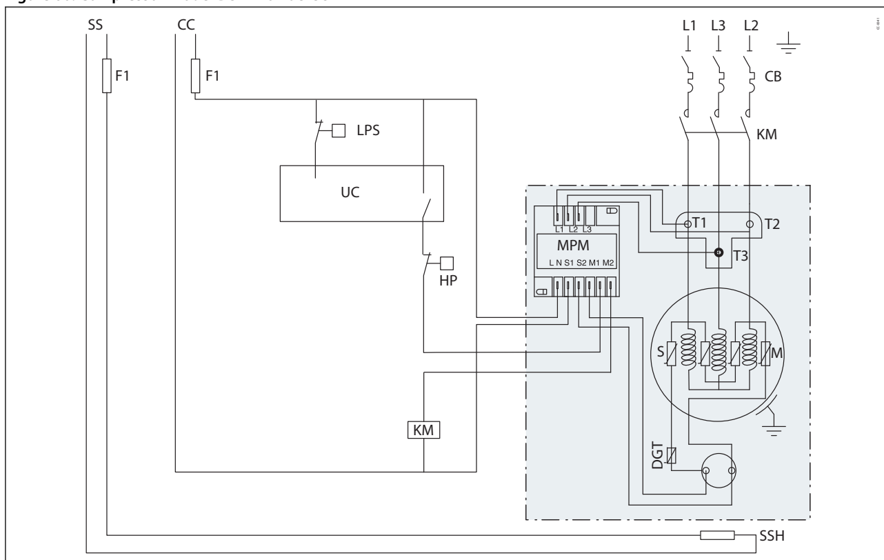
Figure 60: Compressor model DSH240-295-381
