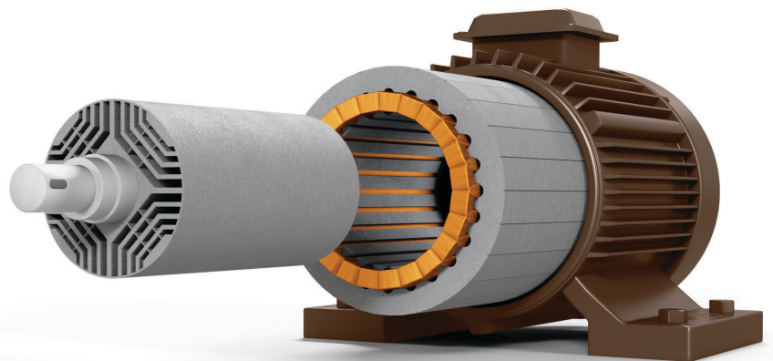
Synchron-Reluktanzmotor
