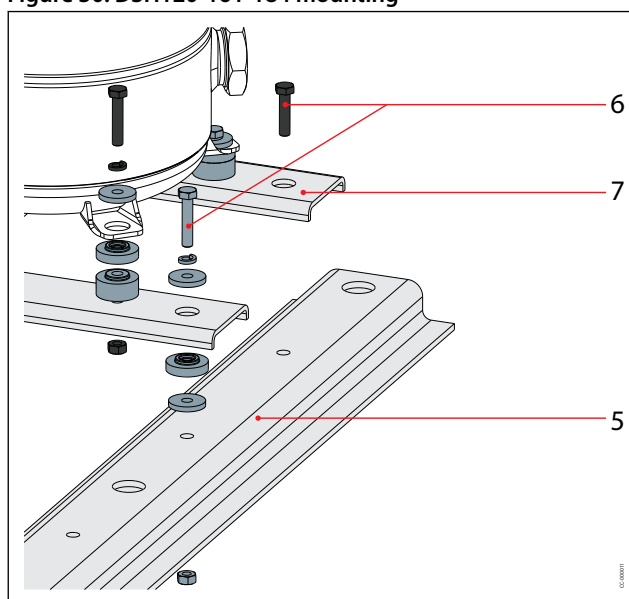
Figure 30: DSH120-161-184 mounting
