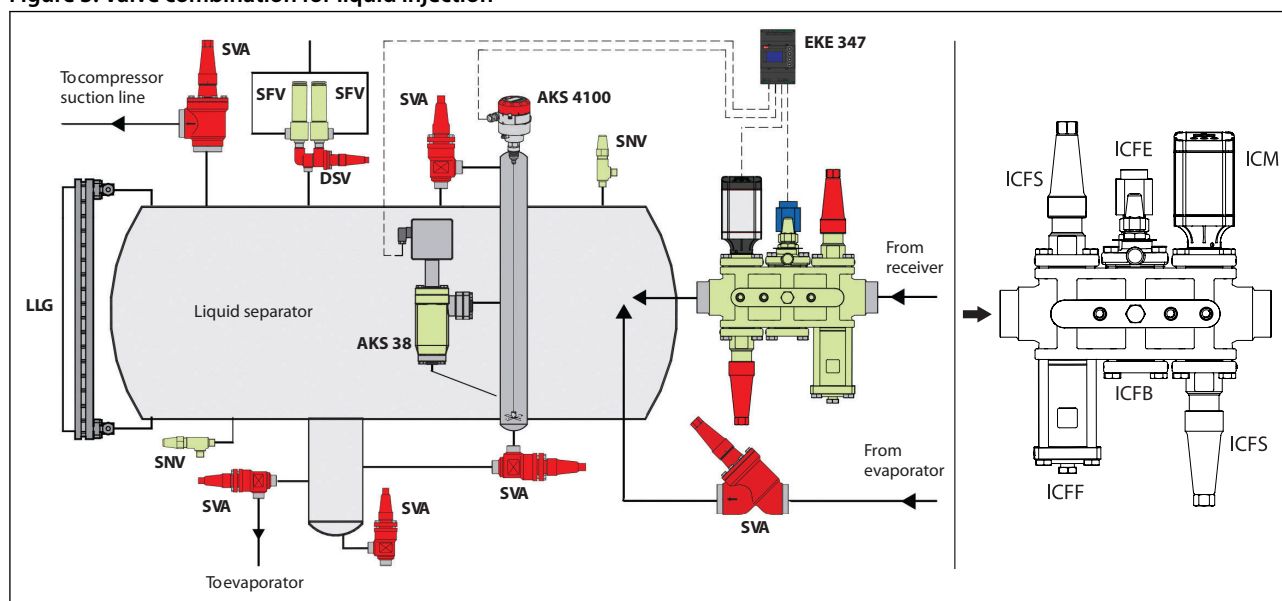
Figure 3: Valve combination for liquid injection
