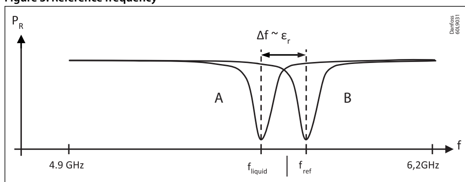
Figure 3: Reference frequency
