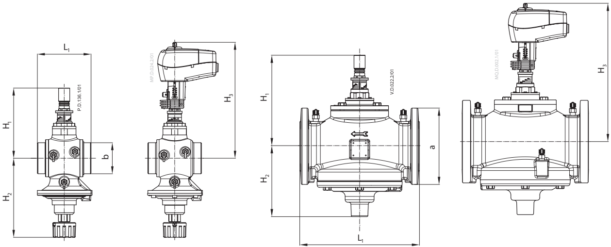
AB-QM DN 40, 50
