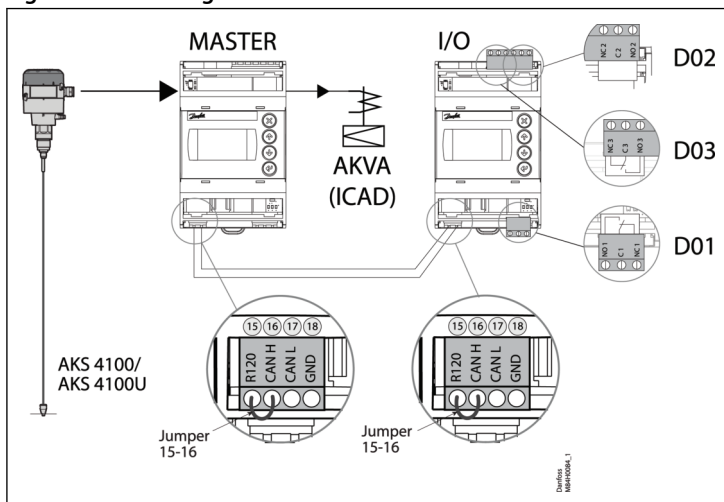
Figure 14: I/O configuration
