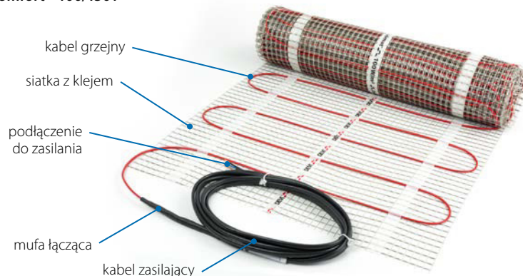
Mata grzejna DEVI comfort ™ 100/150T
