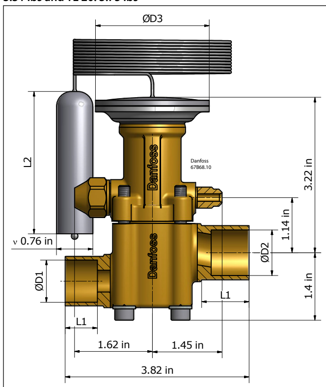
Figure 9: TE 12 and TE 20 Solder straightway, Weight: TE 12: 3.31 lbs and TE 20: 3.75 lbs
