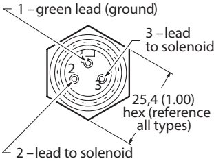
5 pin connector
