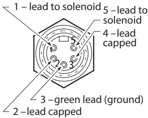
5 pin connector
