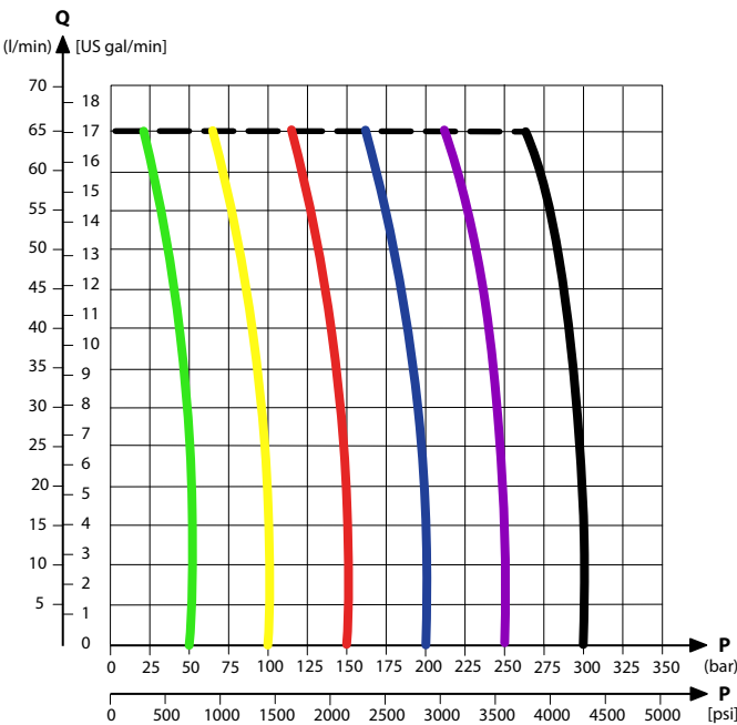
PVB pressure compensated for LS A/B characteristics
