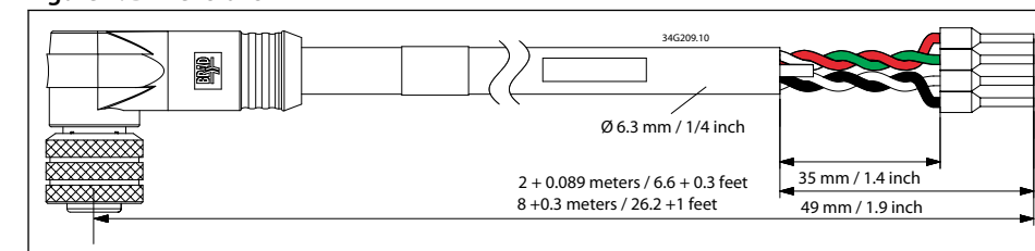
Figure 7: Dimensions
