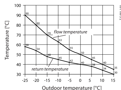
Fig. 3 Return temperature curve graphs
