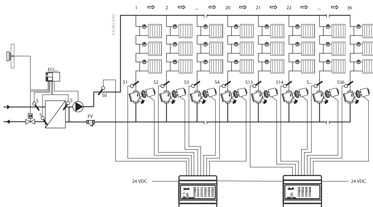
Fig. 2 CCR3+ Controller: scheme with 36 risers
