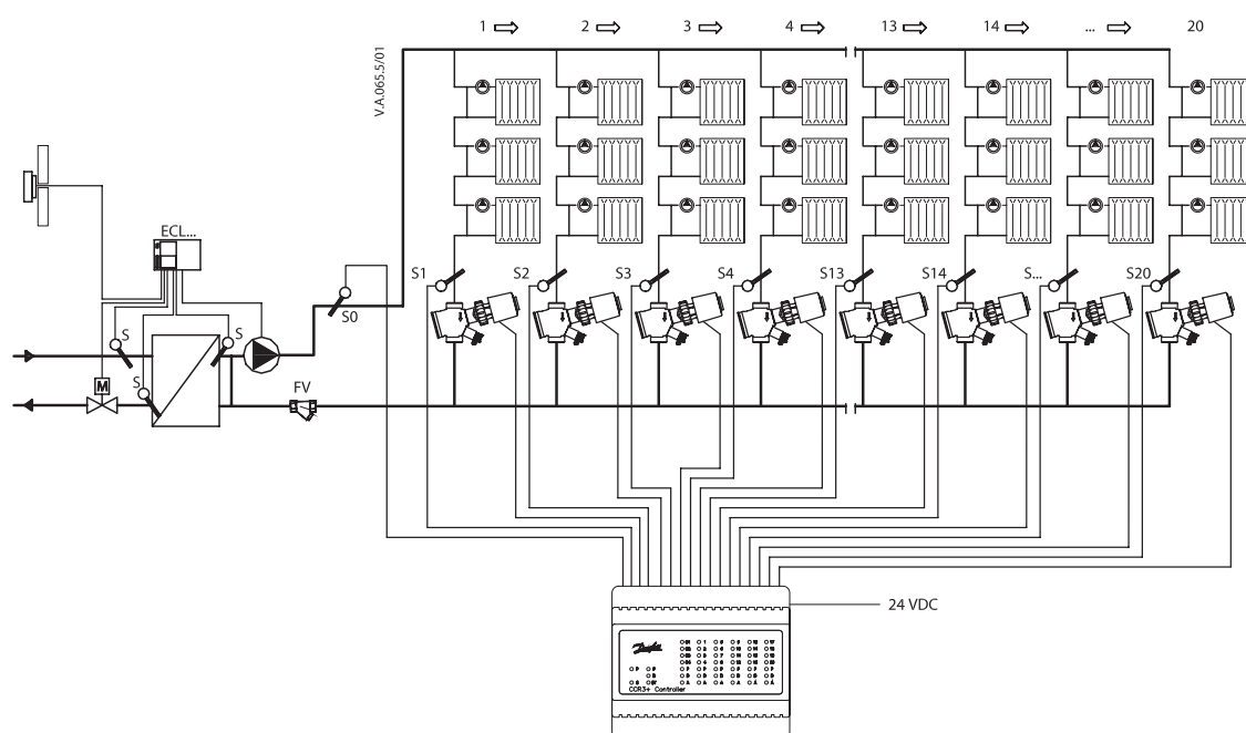
Fig. 1 CCR3+ Controller: scheme with 20 risers
