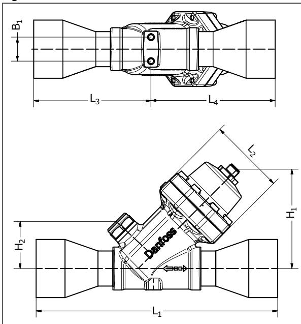
Figure 9: Dimensions ETS 400L
