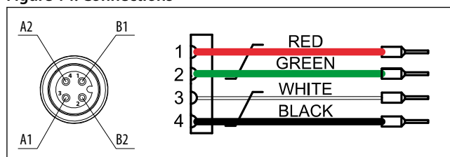
Figure 14: Connections
