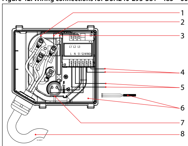
Figure 42: Wiring connections for DSH240-295-381*-485* -600 (*except code 3)
