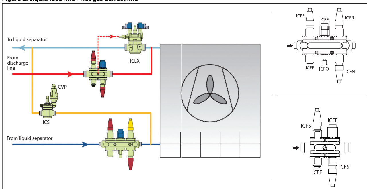
Figure 2: Liquid feed line / Hot gas defrost line
