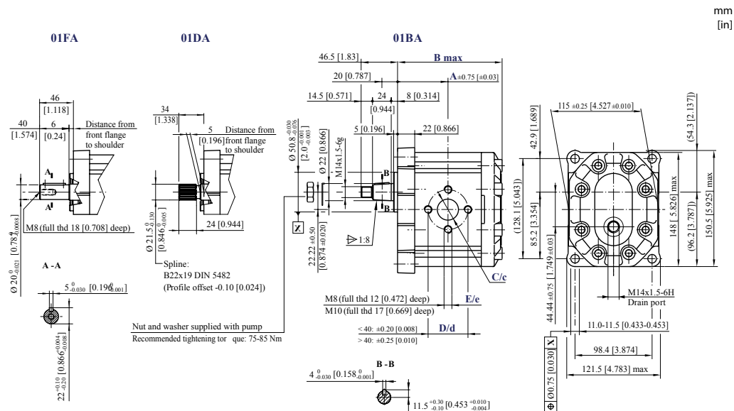
Bidirectional motors dimensions – 01FA, 01DA and 01BA
