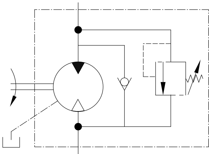
Valve schematic diagram
