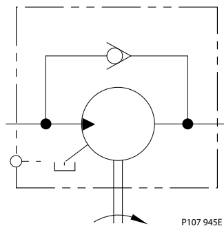
Schematic: Motor with anti-cavitation check valve
