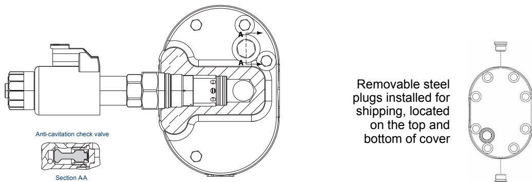
Relief valve cutaway
