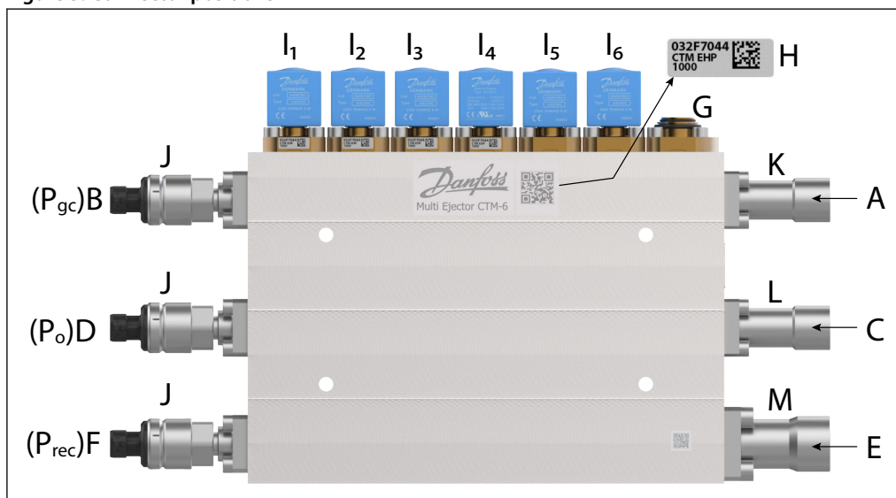
Figure 5: Connector positions
