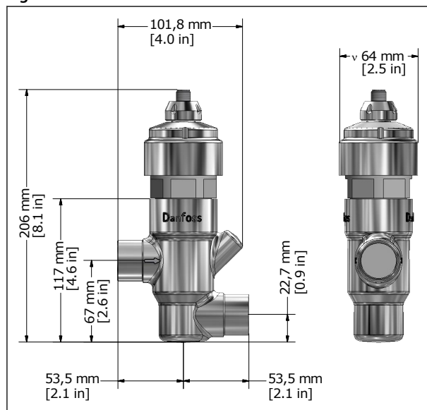
Figure 5: CCMT 16 – CCMT 42
