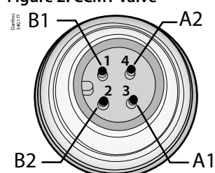
Figure 2: CCMT valve
