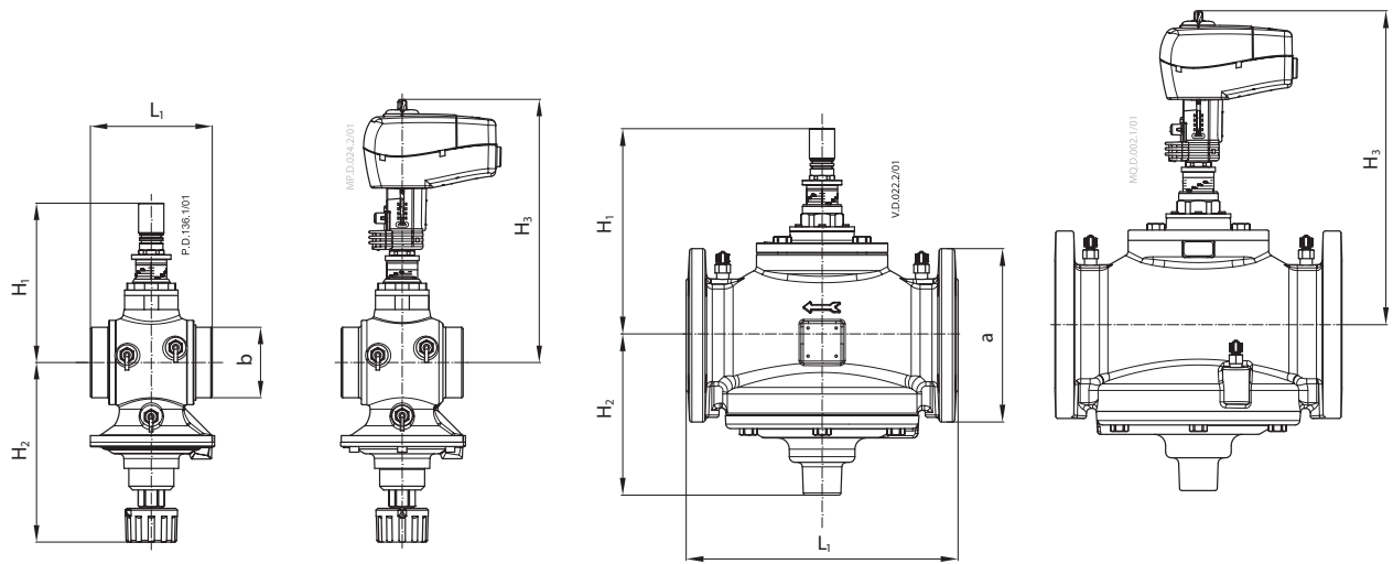
AB-QM DN 40, 50
