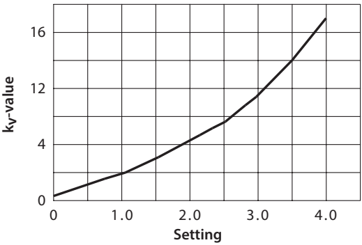
Flow characteristics
