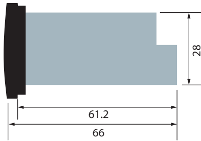
Rear mounting (lock with clips)
