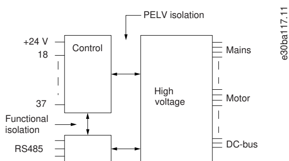
Illustration 51: PELV Isolation
