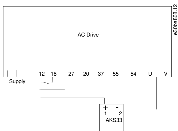
Illustration 46: How to Connect the FC 103 and AKS33 for Closed-Loop Applications
