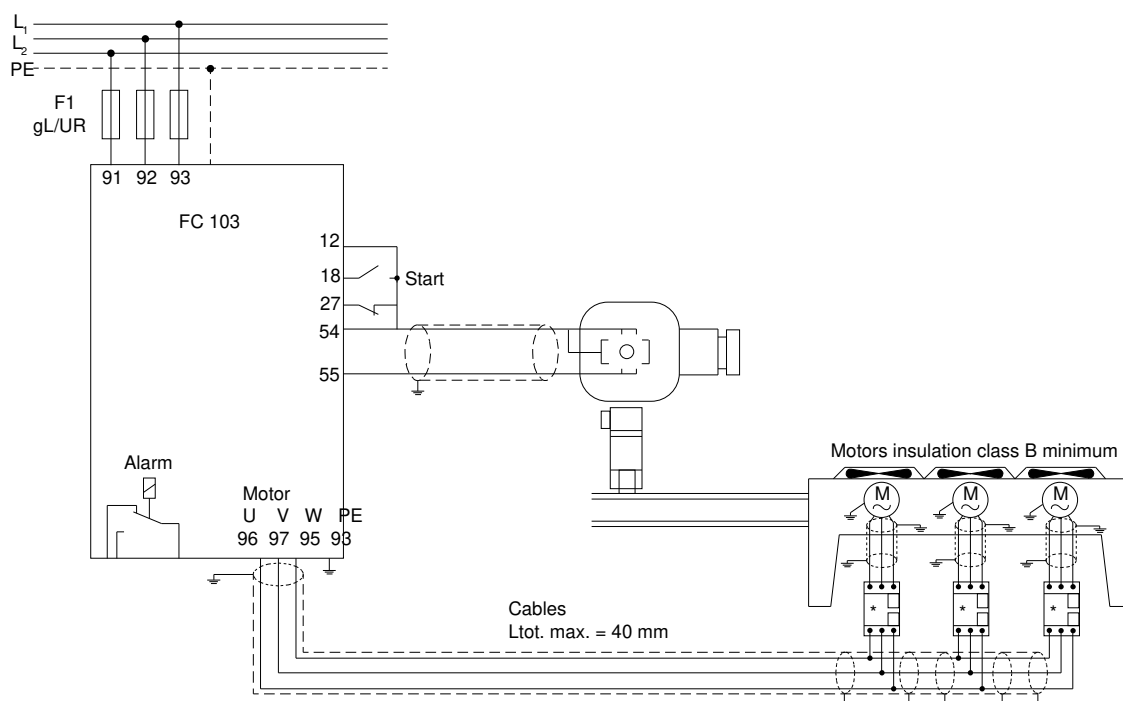
Illustration 44: Pressure Control in Closed Loop – Standalone System - Single Fan or Pump/Multiple Fans or Pumps in Parallel
