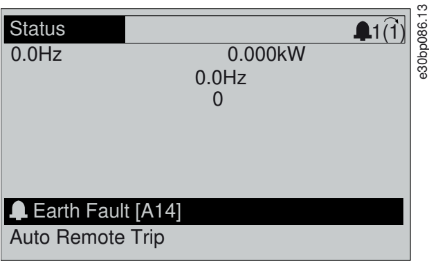
Illustration 50: Alarm Example
