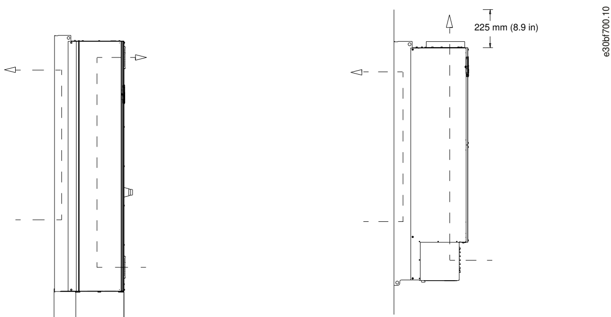
Illustration 69: Airflow Using Back-wall Cooling Kits on E1h/E2h (Left) and E3h/E4h (Right)
