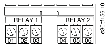
Illustration 34: Relay 1 and Relay 2 Terminals
