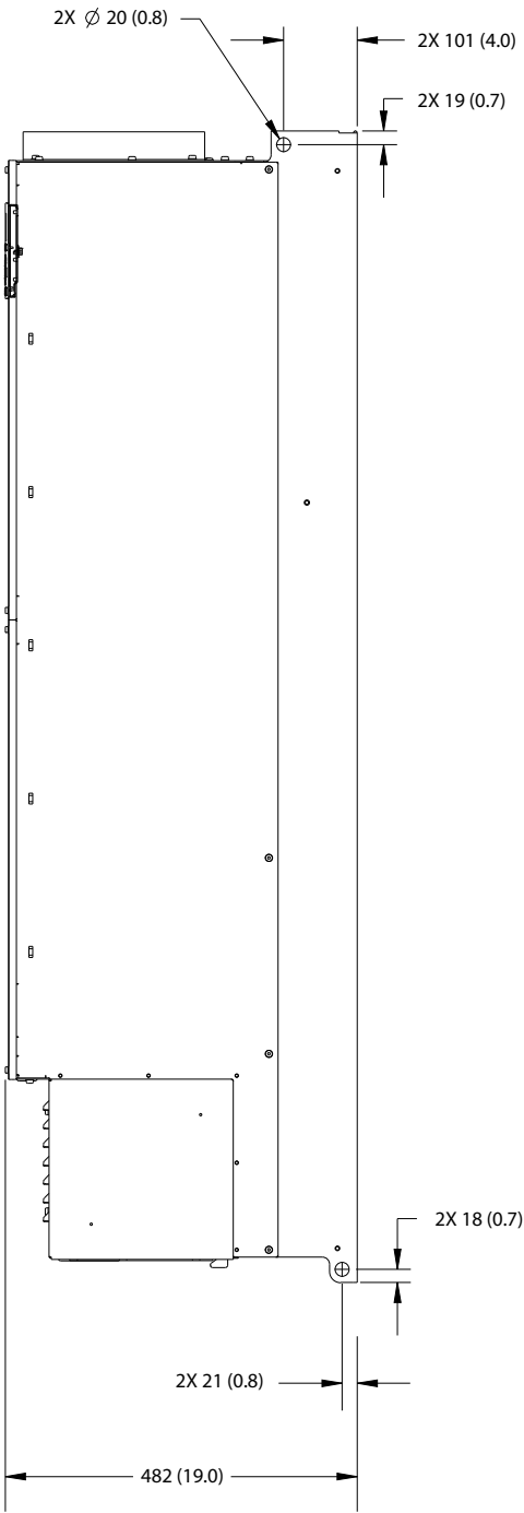
Illustration 61: Side View of E3h
