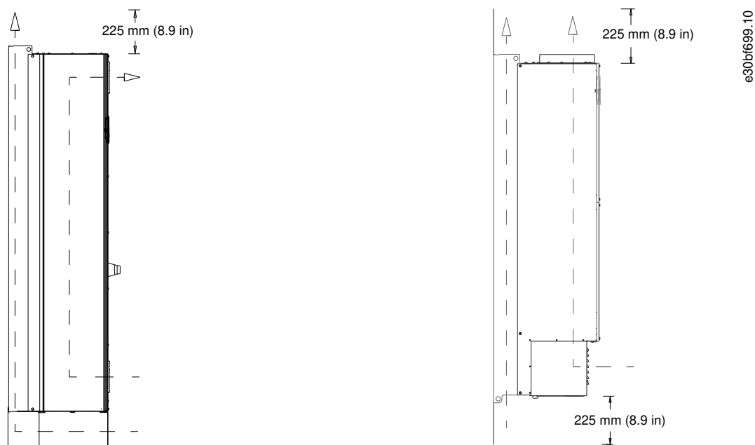
Illustration 68: Airflow for E1h/E2h (Left) and E3h/E4h (Right)
