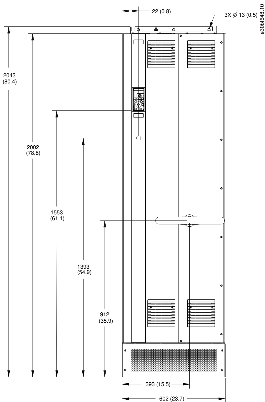
Illustration 52: Front View of E1h
