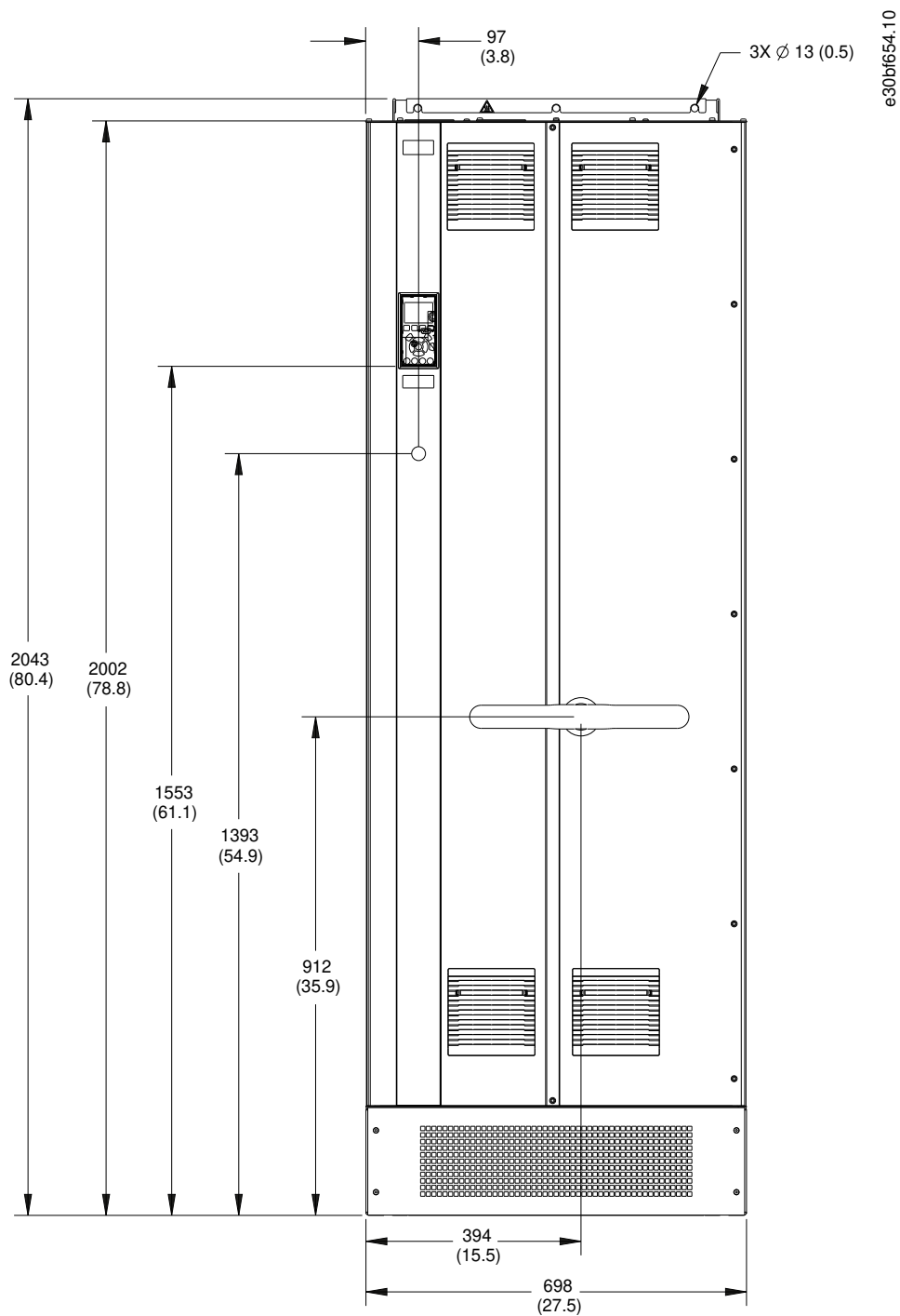
Illustration 56: Front View of E2h
