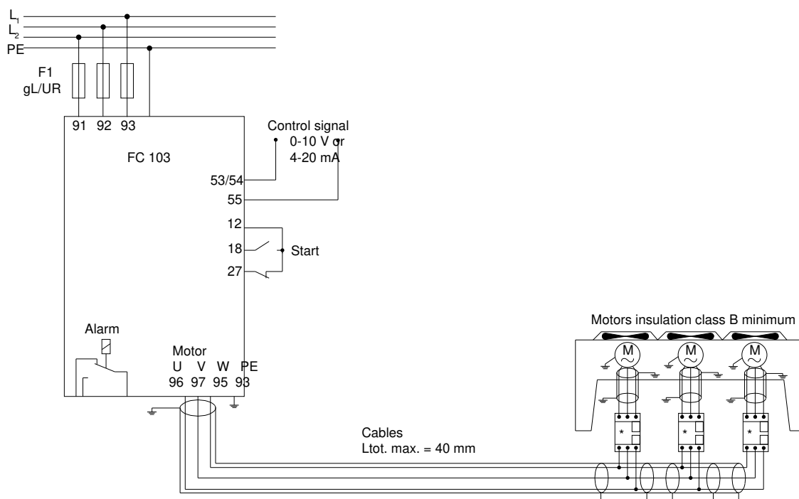
Illustration 43: Speed Control Using Analog Reference (Open Loop) – Single Fan or Pump/Multiple Fans or Pumps in Parallel
