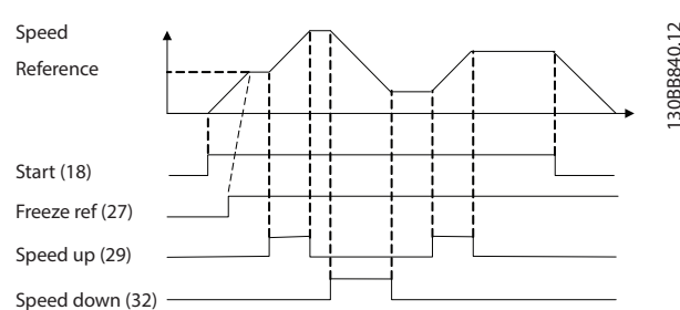
图 6.1 Speed Up/Speed Down
