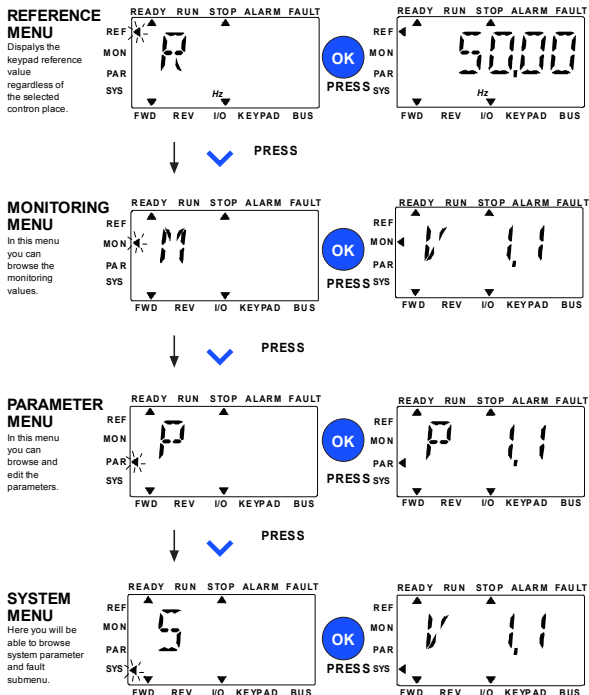
Figure 19: Menú principal de Vacon 20
