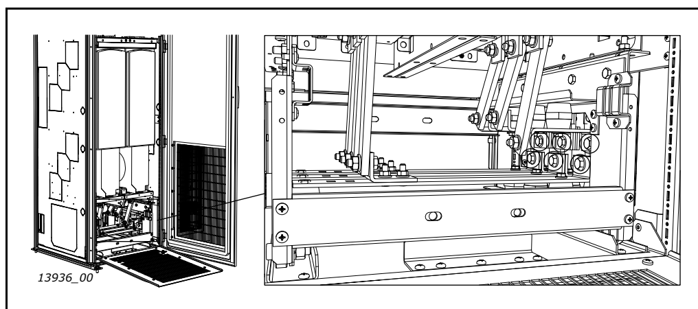
Figure 42. Output busbar mounting screws
