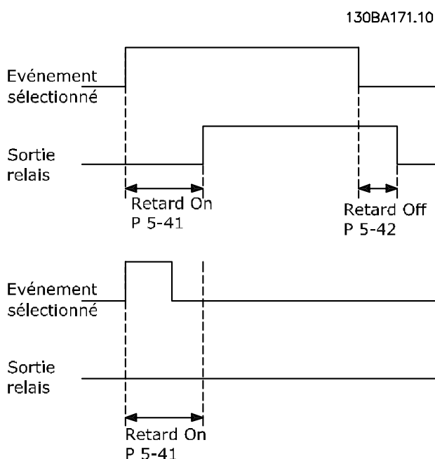
Illustration 4.10 Relais, retard ON
