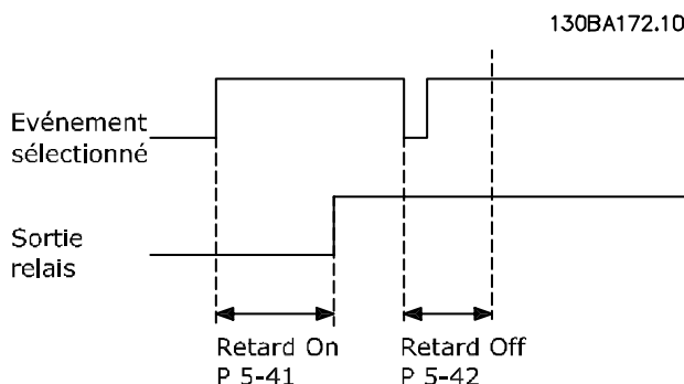
Illustration 4.11 Relais, retard OFF
