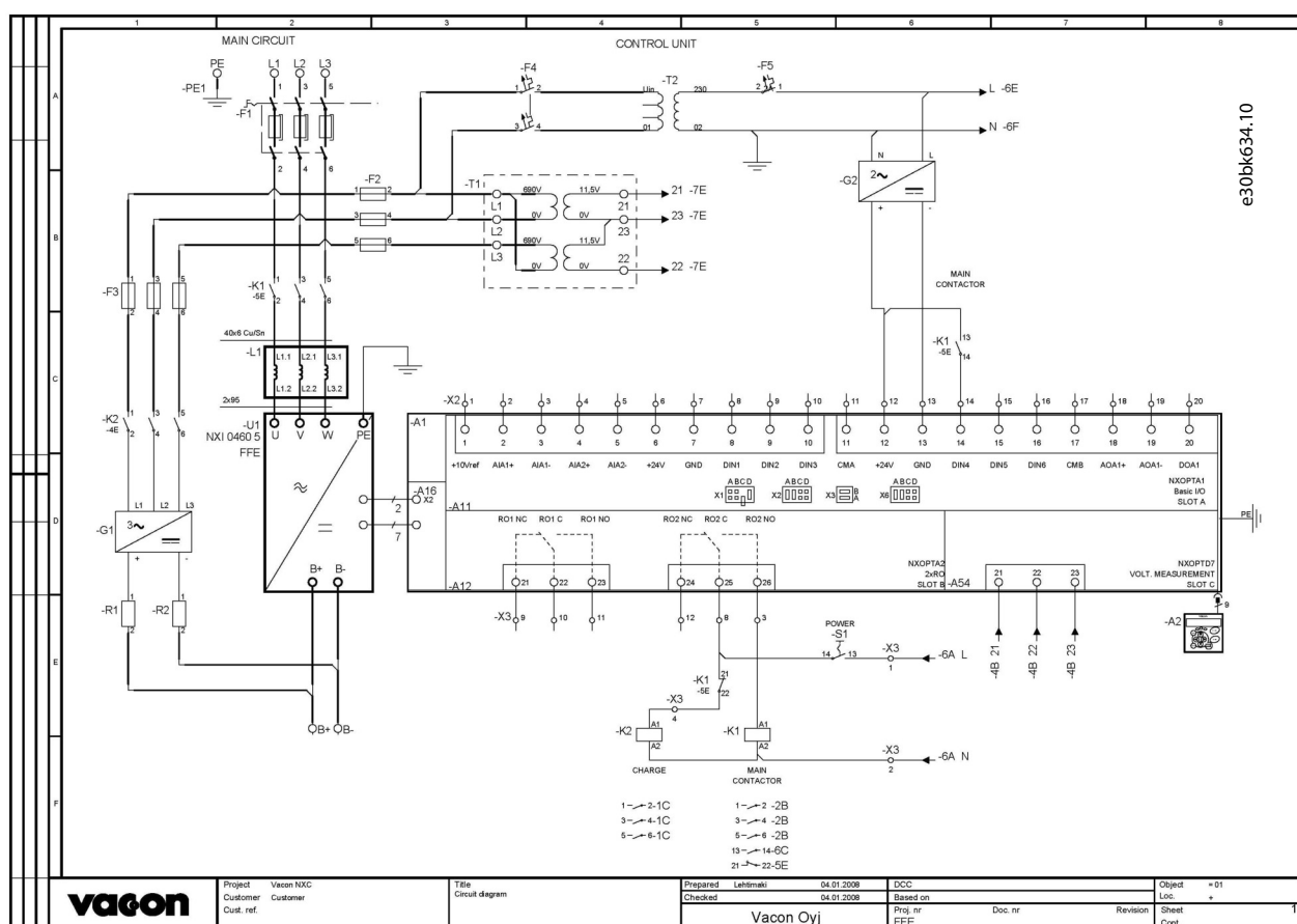
Illustration 5: Connection in FFE Applications
