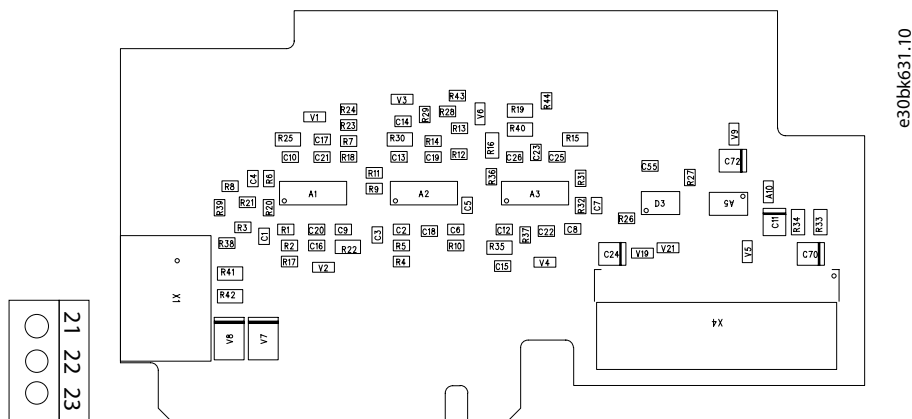
Illustration 1: OPTD7 Option Board Layout
