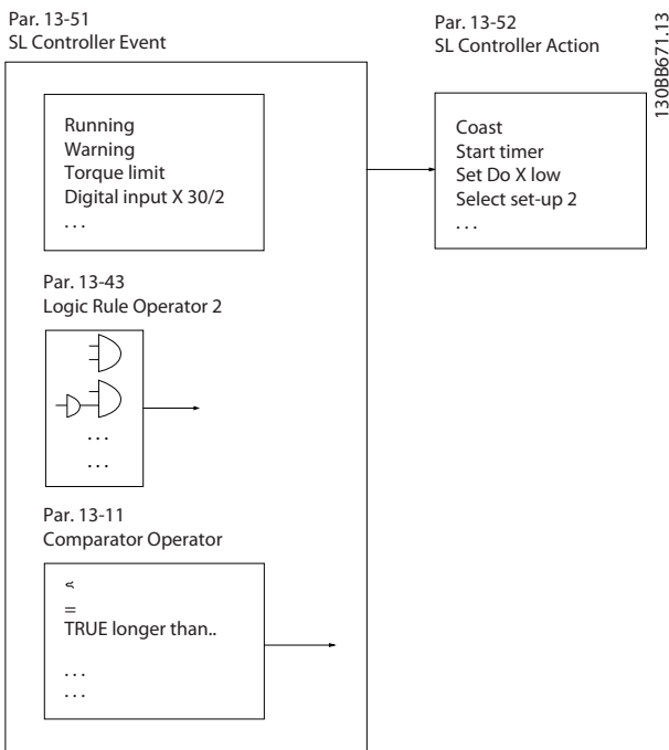
Abbildung 3.52 Smart Logic Control (SLC)
